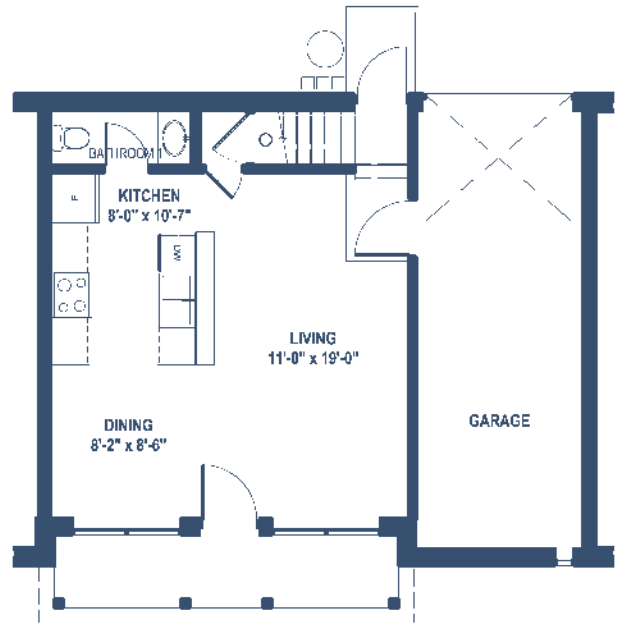
Lower Floor
